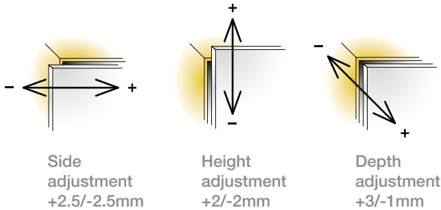
Door adjustment
