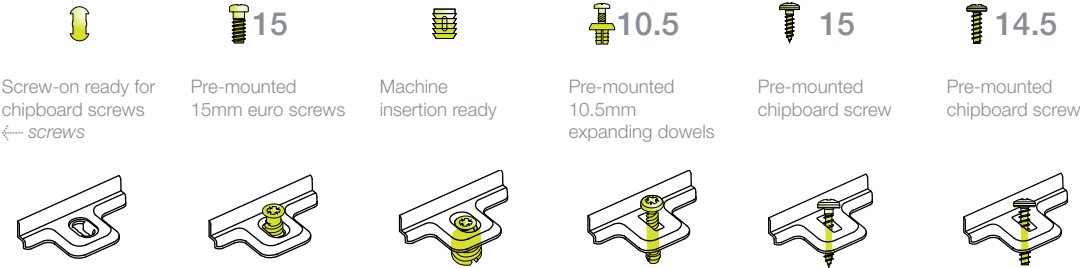
Legend of mounting plate type symbols
