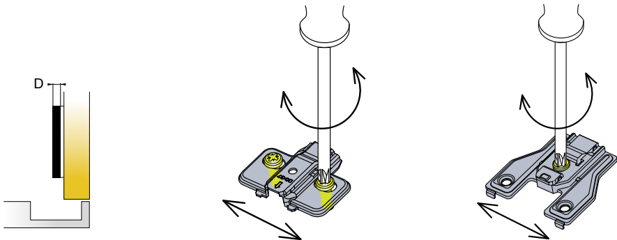
Mounting plate thickness Height adjustment +2/-2mm Height adjustment +2/-2mm
